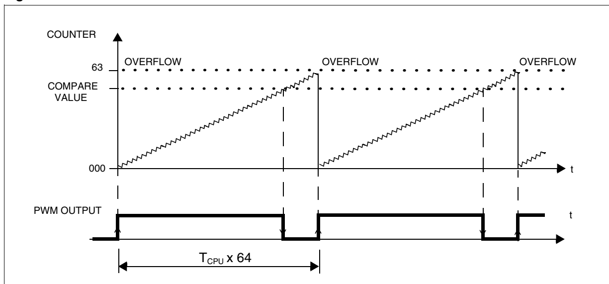
Figure 48. PWM Generation
